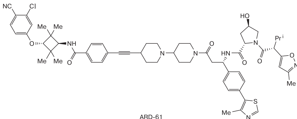
ARD-61
