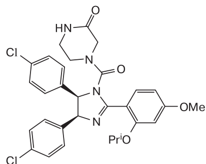
Nutlin-3
